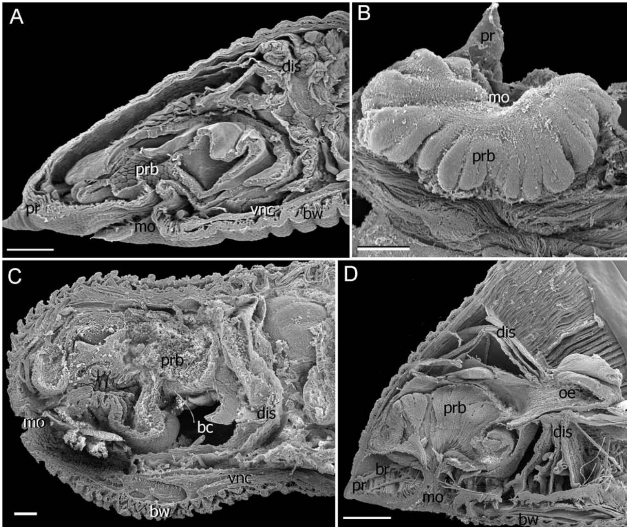
FIGURE 3. SEM. A–B, Travisia forbesii . A, sagittal section with inverted proboscis; B, dissection of anterior part, view of proboscis from the body cavity; C, T. grandulosa , sagittal section with inverted proboscis; D, T. pupa , sagittal section with inverted proboscis. Scale: A = 300 \mu m, B = 400 \mu m, C = 100 \mu m, D = 1 mm. Abbreviations: bc, body cavity; bw, body wall; br, brain; dis, anterior dissepiments (septa); mo, mouth opening; oe, esophagus; po, proboscis opening; pr, prostomium; prb, proboscis; vnc, ventral nerve cord.
