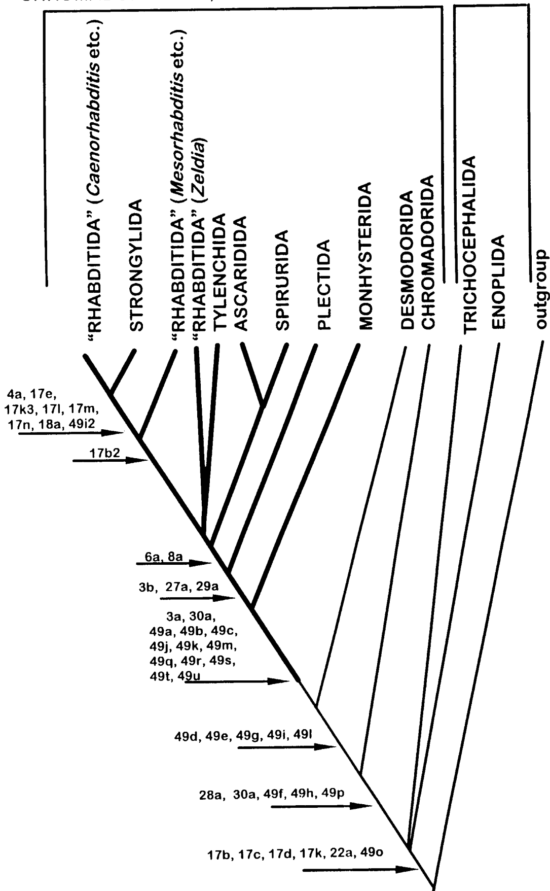
Fig. 6. Summary phylogram depicting the phylogeny of the nematode taxa studied. This tree illustrates a consensus of trees generated by NJ, MP, and ML methods. Arrows indicate the branches where synapomorphic nucleotide substitutions have arisen. Synapomorphies from hairpin regions of 18S rRNA are indicated by corresponding numbers.
